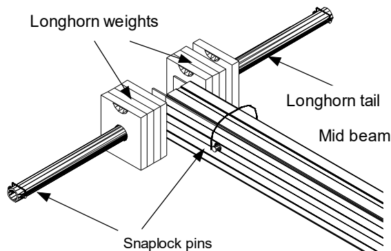
Mid Beam holding Longhorn Weights
