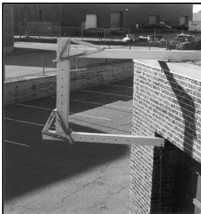
Overhang Beam
