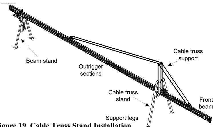
Figure 19. Cable Truss Stand Installation
