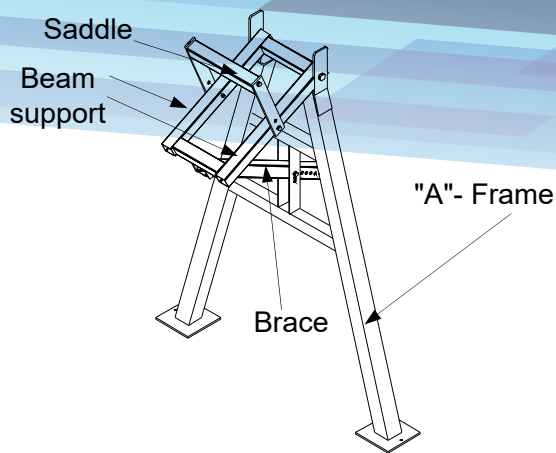
Figure 5. Beam Stand
