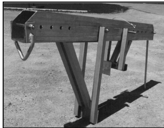
Parapet Clamp
