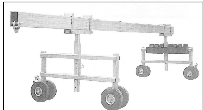
Beam Dollies
