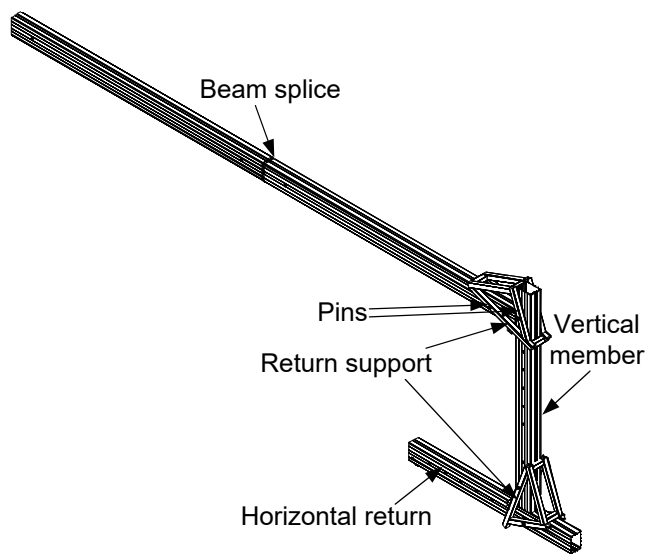
Figure 21. Overhang Beam
