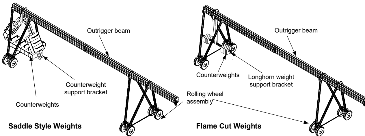
Figure 24. Rolling Outrigger
