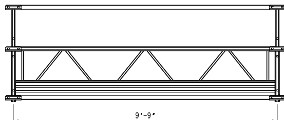
10 feet section – 3 meter section
